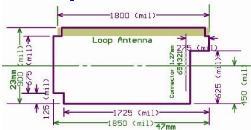
RMB-500UHF Series Receiver PCB size keepout Yoyang Inc Taiwan Y6170227044
